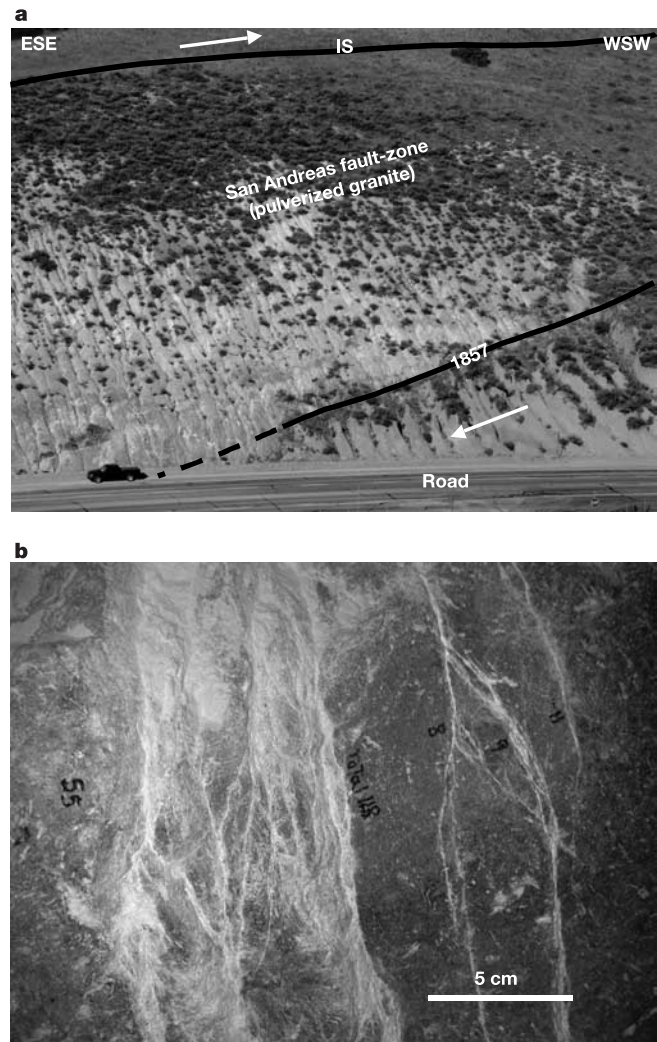
Figure 1 Field setting of the investigated faults. a , The San Andreas fault-zone at Tejon Pass, California. The car is shown for scale. IS, inactive fault segment; 1857, slipping segment of the 1857 earthquake. Note the gouge zone 70–100 m wide with badland morphology of the pulverized granite. This exposure and its extensions were mapped, and hundreds of gouge samples were collected. b , Close-up view of the fractured zone of the Bosman fault (text). The white striations are coalescing fractures filled with gouge powder (rock flour) that cut across the solid, dark quartzite.
